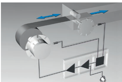
Open-loop controlled with \varnothing -calculation
